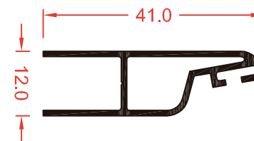
LEX10924 LAMA TERMINAL 41 MM
