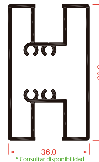
LEX3102 HOJA MALLORQUINA PLEGABLE
