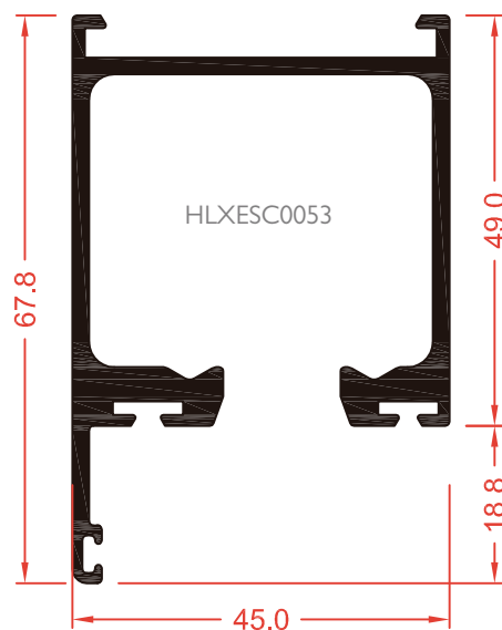
LEX3100 MARCO SUPERIOR PLEGABLE
