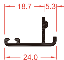
LEX3105 BATIENTE PLEGABLE
